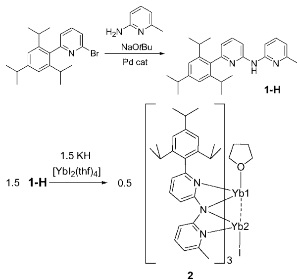
Scheme 1. Synthesis of 1 and 2 .
